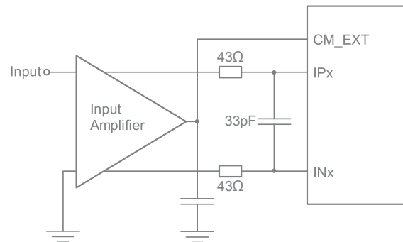
Figure 10. DC-Coupled Input
