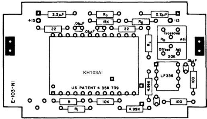
Figure 8: Component placement guide, non-inverting
