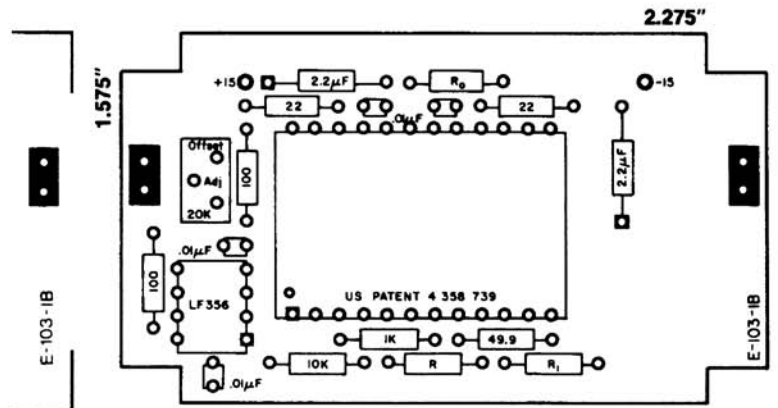
Figure 4: Component placement guide, inverting
