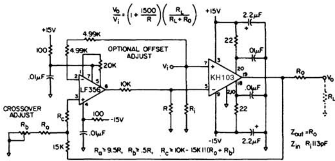
Figure 5: Non-inverting circuit with offset adjust circuitry
