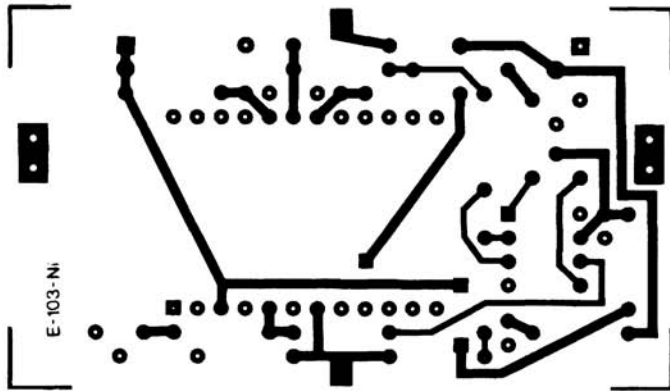
Figure 6: Component side (top), non-inverting
