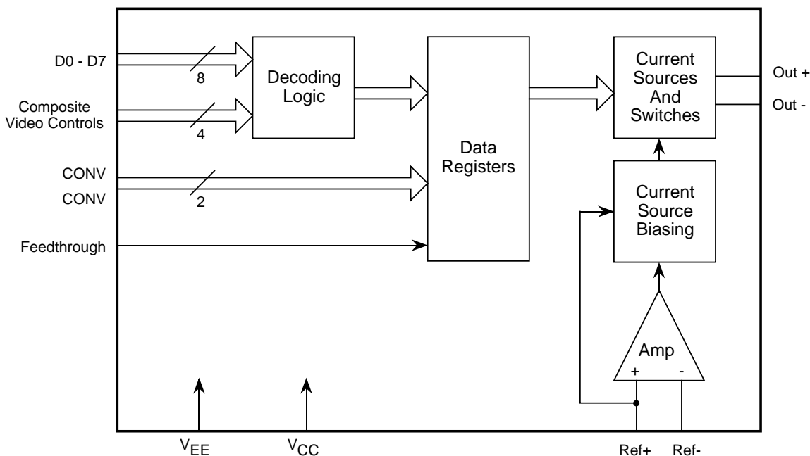
Figure 1 - Functional Diagram
