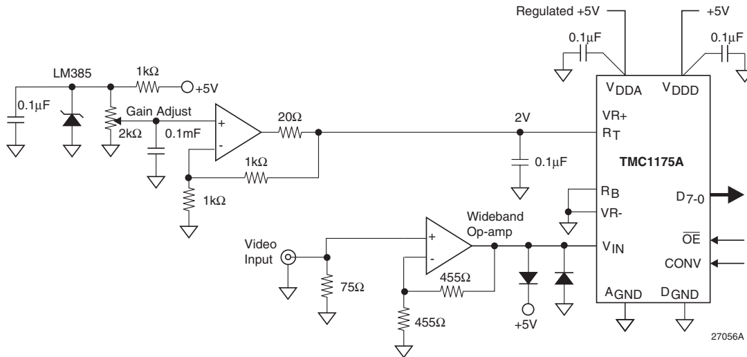
Figure 12. Typical Interface Circuit-High Performance
